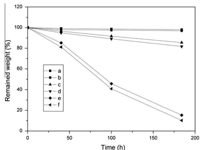
Fig. 6. Remained weight of the blank PLLA fiber and F1 sample in PBS, PBS with 10 mg/L proteinase K and PBS with 50 mg/L proteinase K (weight was the average of triplicate samples) (curve a: blank PLLA fiber in PBS, curve b: F1 fiber in PBS, curve c: blank PLLA fiber in PBS with 10 mg/L proteinase K, curve d: F1 fiber in PBS with 10 mg/L proteinase K, curve e: blank PLLA fiber in PBS with 50 mg/L proteinase K, curve f: F1 fiber in PBS with 50 mg/L proteinase K).
