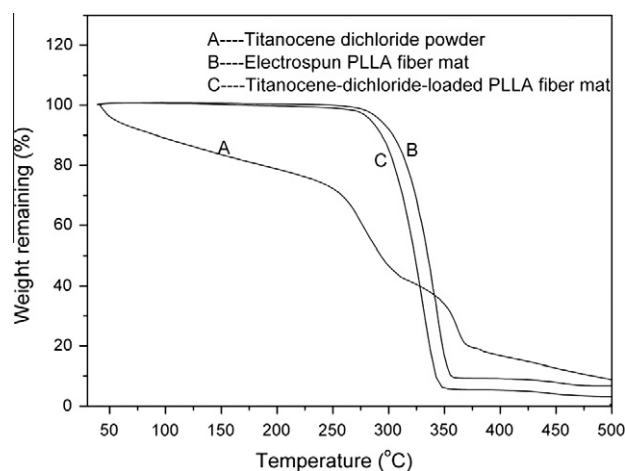
Fig. 3. Thermogravimetric analytical thermograms of the products: (A) titanocene dichloride powder, (B) electrospun PLLA fibers and (C) titanocene-dichloride-loaded PLLA fiber mat (heated from 40 to 500 °C at a heating rate of 10 °C/min).
