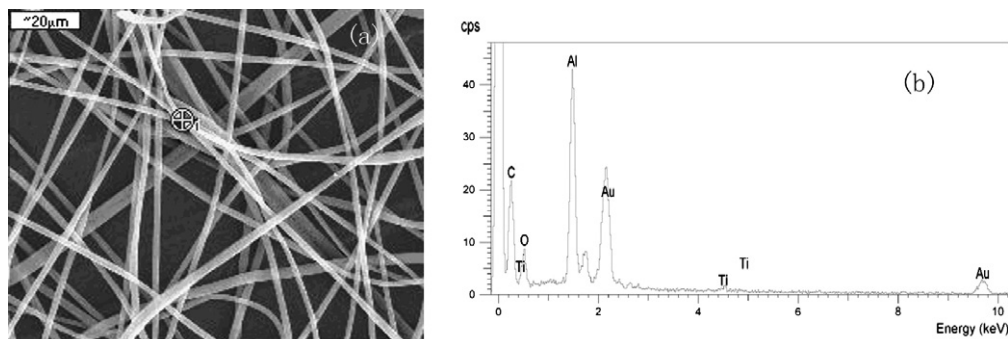
Fig. 1. SEM micrograph (a) and EDS micrograph (b).
