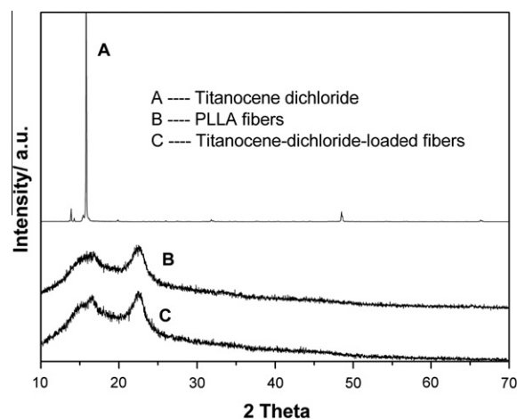
Fig. 2. XRD patterns of the samples: (A) titanocene dichloride powder, (B) PLLA fibers and (C) titanocene-dichloride-loaded PLLA fibers.
